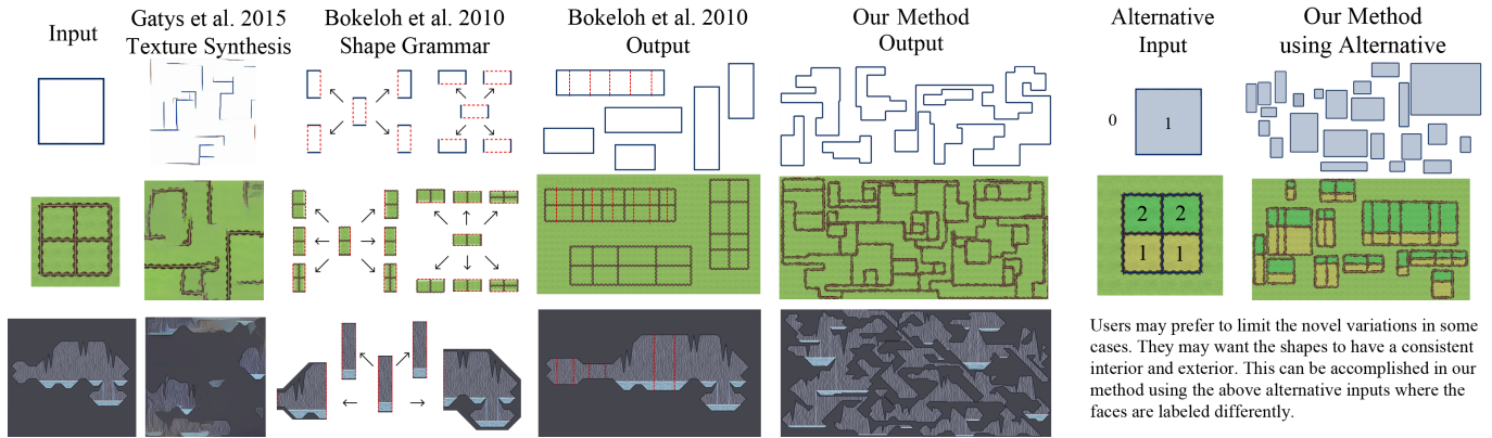
Fig. 10. Prior work has trouble with loops. Existing methods either do not close the loops [Gatys et al. 2015] or they directly copy the input with only minor changes to the aspect ratio [Bokeloh et al. 2010]. The red lines in Bokeloh et al.’s grammar are their docking sites.
