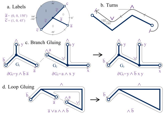
Fig. 3. (a) Face and edge labels. (b) Positive \wedge and negative \vee turns for paths. (c,d) Graphs are assembled by gluing half-edges together. The opposite of gluing is cutting. Each graph G has a boundary string \partial G .
