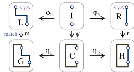
Fig. 7. A double-pushout production rule. The left side L is matched with G . L is cut from G and R is glued in its place to make H .
