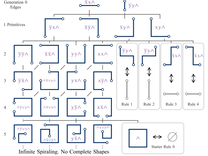
Fig. 5. A graph hierarchy starts simple and grows more complex as primitives and loops are glued. From the hierarchy, a graph grammar with five rules is found by matching boundary strings.
