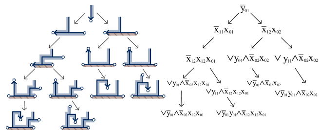
Fig. 12. A decision tree of possible gluing operations starting with \overline{y_{01}} .
