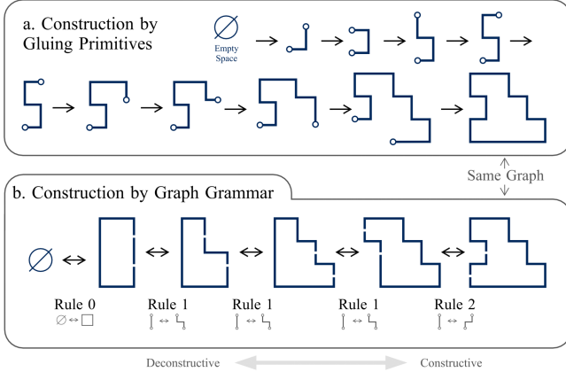
Fig. 6. One way of constructing graphs (a) is to randomly glue primitives together until the graph is complete. A better way is to use a graph grammar (b). Fig. 5 shows how this graph grammar is automatically generated.
