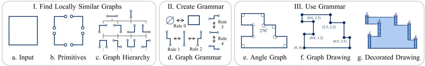
Fig. 2. Overview. The input shape (a) is cut into primitives (b). Primitives are glued into new graphs which are organized into a hierarchy (c). From this, a graph grammar (d) is constructed that generates angle graphs (e). Vertex positions are added to create a graph drawing (f) and decorations can be added (g, optional).
